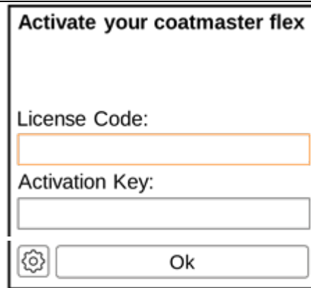
Figure 14: Activating menu
